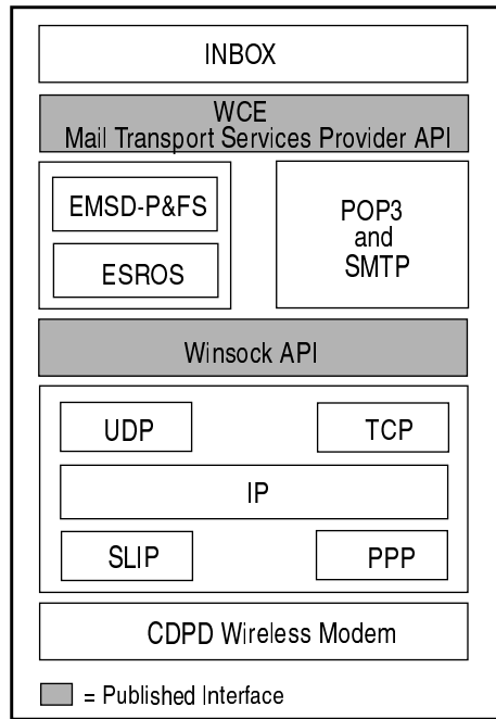
Figure 1: Components of WCE Mail Transport Service Provider with EMSD
