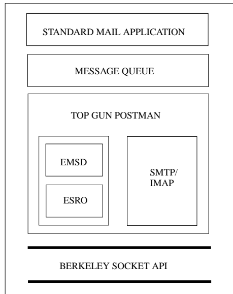
Figure 1: Example of Separate Mail Transfer Service for Palm OS
